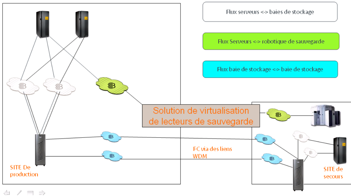
Figure 18 - architecture SAN - étape 3
