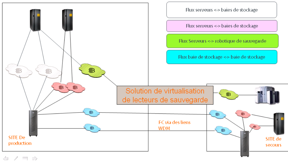
Figure 17 - architecture SAN - étape 2
