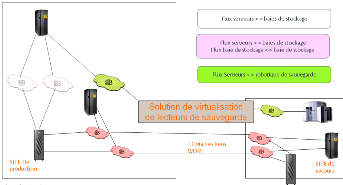
Figure 16 - architecture SAN - étape 1
