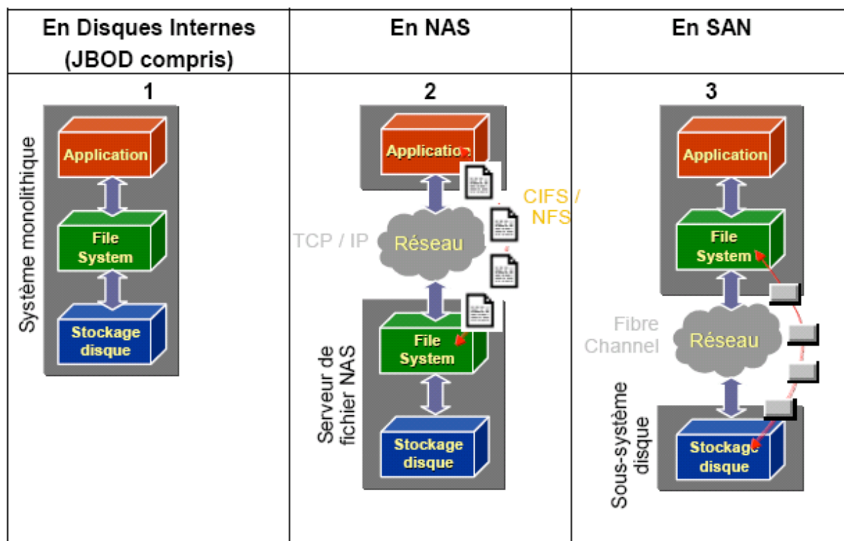
Figure 1 - JBOD vs NAS vs SAN/DAS
