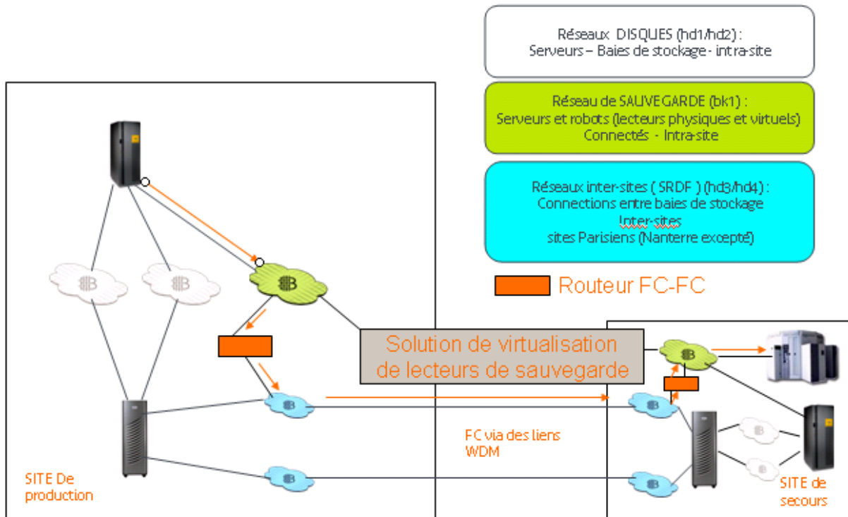
Figure 10 - Architecture SAN 2006-2007 "routé"
