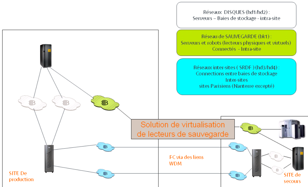
Figure 9 - Architecture SAN 2006-2007
